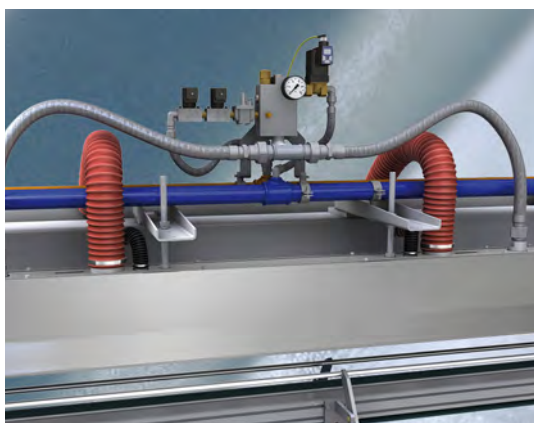
Air - gas mixer unit to SOUCURE LG, for each burner, which allows an individual heat regulation by means of automatic temperature controllers.
